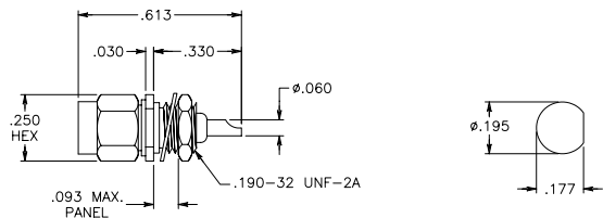
(SMC Plug) Bulk Head Receptacle Front Mount Solder Cup Terminal
