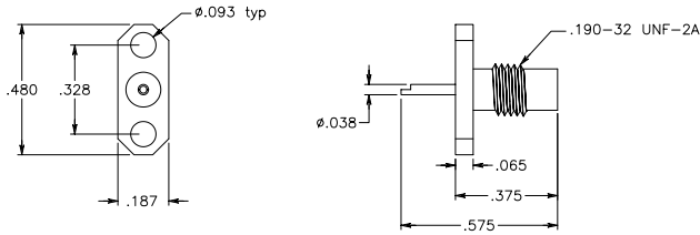
(SMC Jack) 2-Hole Flange Mount Solder Cup Contact
