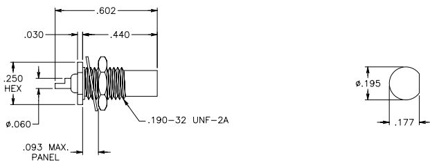
(SMC Jack) Bulk Head Receptacle Rear Mount Solder Cup Terminal
