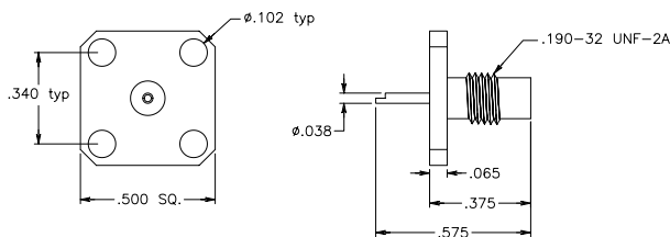
(SMC Jack) 4-Hole Flange Mount Solder Cup Contact
