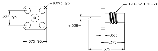
(SMC Jack) 4-Hole Flange Mount Solder Cup Contact
