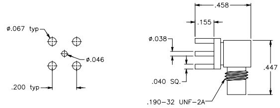
(SMC Jack) Right Angle Printed Circuit Mount
