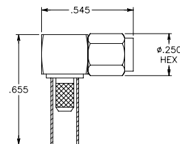
(SMC Plug) Right Angle Crimp Attachment For RG178 & RG196
